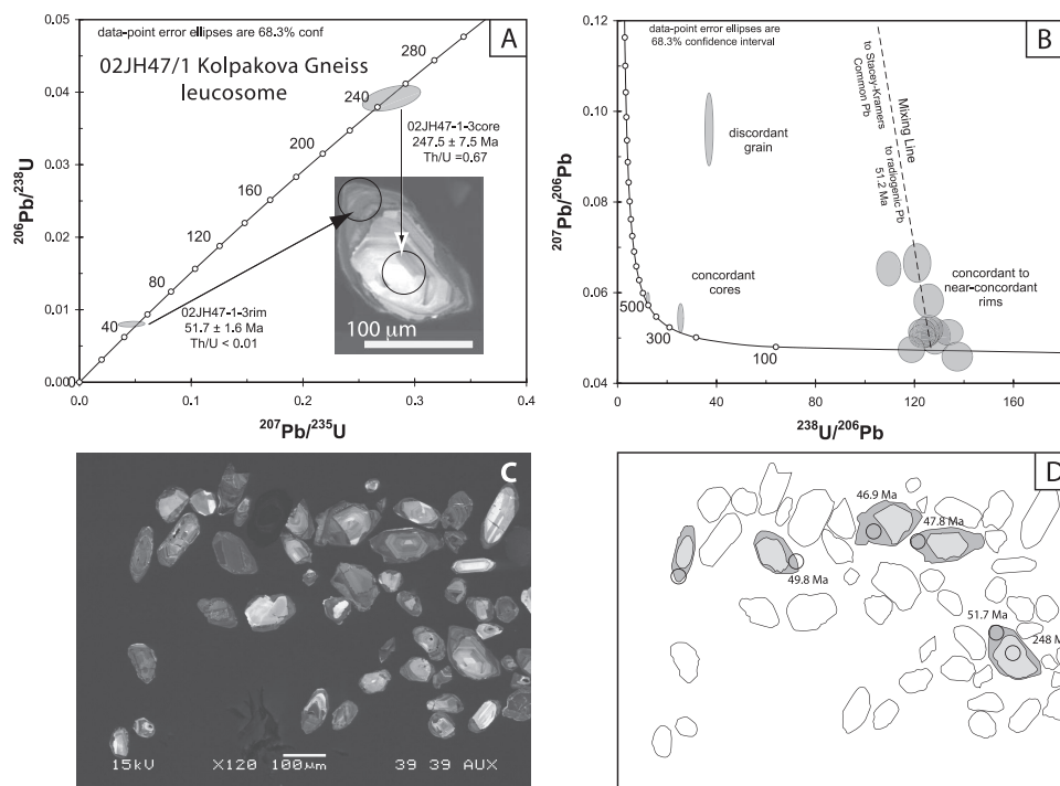
Fig. 14. Plots and CL images for zircons from a leucosomal segregation within the Kolpakova Gneiss (sample 02JH47/1). (A) Wetherill concordia diagram and CL image showing data from a core-rim pair analysis: the core has bright CL with moderate Th/U, crenulate margins and yields a 247 Ma grain-age indicating resorption of a zircon xenocryst; the rim has low CL, low Th/U, is euhedral and yields a 52 Ma grain-age indicating its origin as a metamorphic zircon overgrowth. (B) Analyses of multiple rims (panels C-D) produce a linear mixing array of common Pb and 51.2 \pm 0.5 Ma radiogenic Pb. Isotopic data are presented in Appendix A.8.
