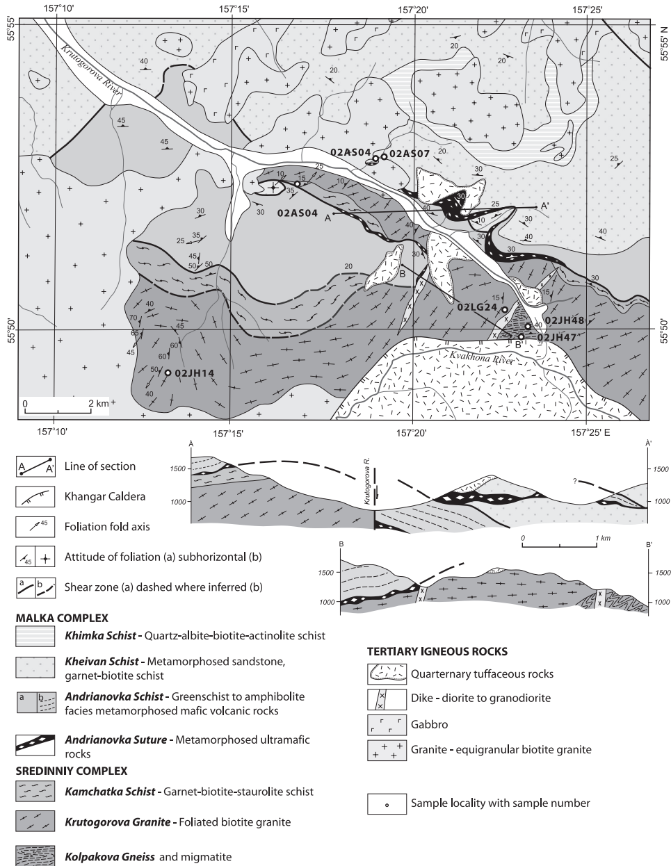
Fig. 4. Geologic and sample locality map and geologic cross sections for the upper Krutogorova River watershed study area (modified from Rikhtyer, 1995).
