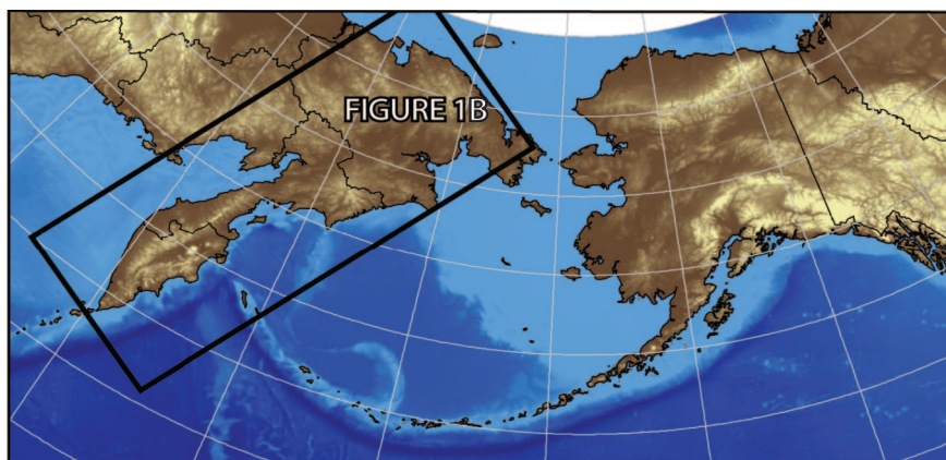
Fig. 1.(A) Index map. Shows the location of the geologic map area in figure 1B.
