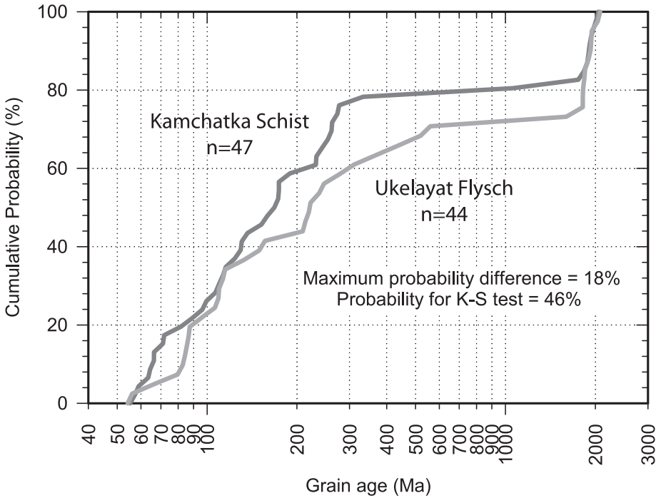
Fig. 23. Comparison of cumulative probability distributions for U-Pb grain-ages of the Kamchatka Schist and Ukelayat Group samples. The Kolmogorov-Smirnov statistic ( P(KS) ) is a nonparametric test of the degree of misfit of two independent populations. Here P(KS) = 46\% indicates the probability that the difference between the two distributions might occur by chance alone.
