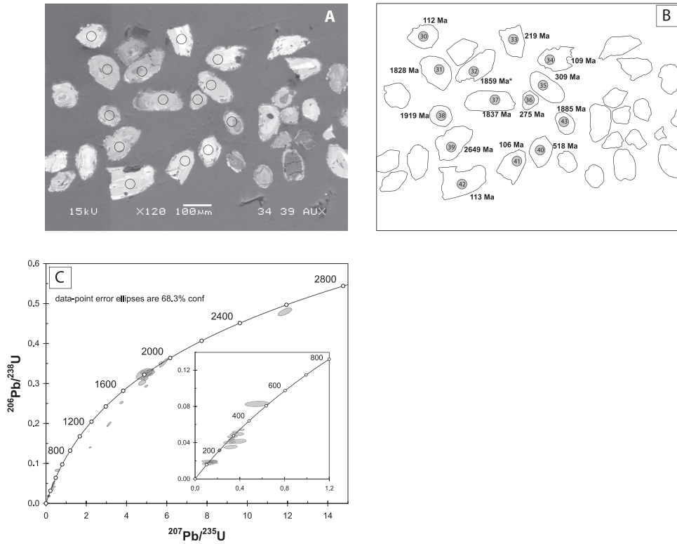
Fig. 10. Wetherill concordia, CL image and summary grain-age diagram for detrital zircons of the garnet-biotite Kamchatka Schist (sample 02AS07) from the upper Krutogorova watershed (fig. 5). (A) CL image showing location of spot analyses, age data are given in Appendix A.4. (B) Rounding is evident in these grains although the crenulate margins of some grains suggest minor dissolution prior to precipitation of zircon overgrowths. (C) Wetherill concordia diagram showing isotopic data. Zircons generally yield concordant grain-ages that range from mid-Cretaceous (106.2 Ma) to Archean (2649 Ma) (see table 5). An Albian maximum stratigraphic age is assigned to the protolith for this unit based on the youngest concordant grain-ages.
