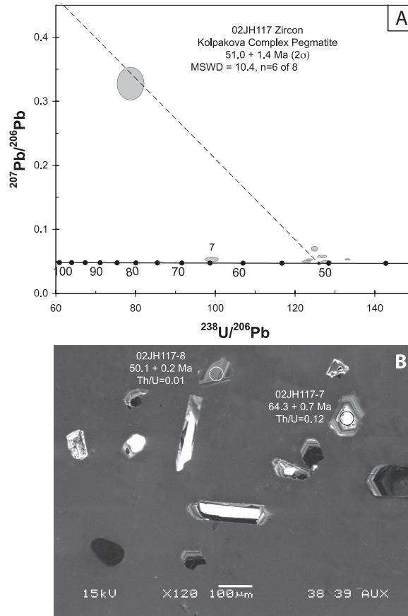
Fig. 15. Tera-Wasserburg concordia plot (panel A) and CL image (panel B) with ^{207}\text{Pb} -corrected ^{206}\text{Pb}/^{238}\text{U} grain-ages for analyzed representative zircons from a boudinaged garnet-muscovite-Ksparg pegmatite (sample 02JH117) within the Kolpakova Gneiss in the Left Andrianovka region. The data exhibit considerable scatter despite textural heterogeneity, perhaps due to Pb loss caused by radiation damage in very high U zircons (Appendix A.9).
