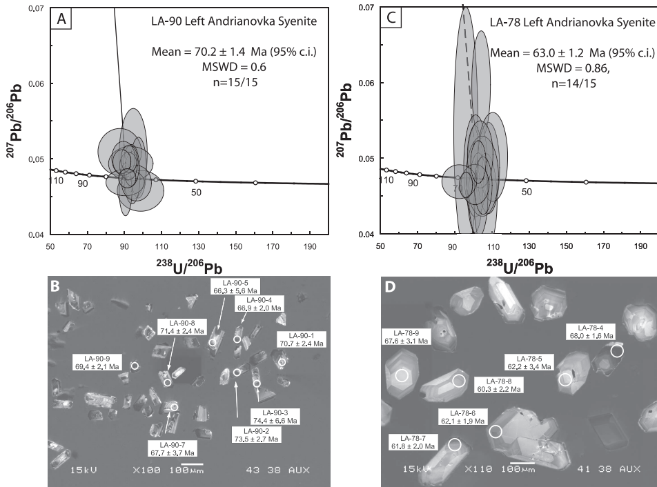
Fig. 12. Tera-Wasserburg concordia plots and CL images with ^{207}\text{Pb} -corrected ^{206}\text{Pb}/^{238}\text{U} grain-ages for texturally representative zircons from syenitic bodies (samples LA-78 and LA-90) within the Left Andrianovka massif, Left Andrianovka River region. Isotopic data are presented in Appendix A.6.
