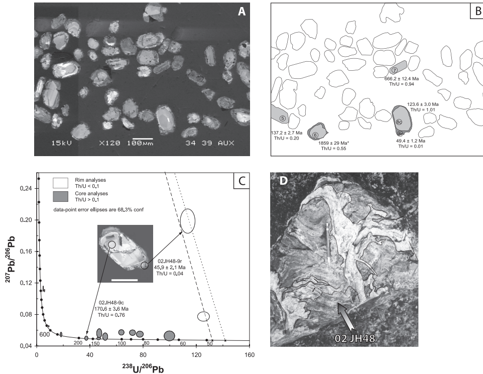
Fig. 8. Single-grain U-Pb data and CL images for zircons from a melanosome of the Kolpakova migmatites (Sample 02JH48) in the upper Krutogorova watershed. (A) Cathodoluminescence image of polished zircons. (B) Outlines of individual grains and position of spot analyses with corresponding ^{207}\text{Pb} -corrected ^{206}\text{Pb}^*/^{238}\text{U} ages. Encircled numbers refer to data in Appendix A.2. Note that analyzed grains have been colored to indicate core and rim domains. Th/U ratios of individual analyses are shown because low Th/U ratios ( <0.01 ) are thought to be a hallmark of zircon overgrowths formed in wet metamorphic conditions (for example, Ireland and Gibson, 1998) consistent with zircon overgrowth formation during migmatization. (C) Tera-Wasserburg concordia plot of all sample 02JH48 data. Filled ellipses are considered primary, detrital ages while open circles represent data from low Th/U relatively higher common Pb metamorphic zircons and zircon overgrowths. (D) Outcrop-scale photograph of migmatites of the Kolpakova Gneiss; sample 02JH48 was taken from the melanosome.
