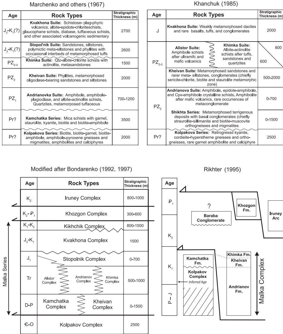
Fig. 3. Summary stratigraphic and tectonostratigraphic columns depicting the evolution of stratigraphic terminology and tectonostratigraphic interpretations for the Sredinnyi Range from the late 1960's to the mid 1990's. This figure is intended to familiarize the reader with the history of research in the Sredinnyi Range documented largely in Russian-only publications.
