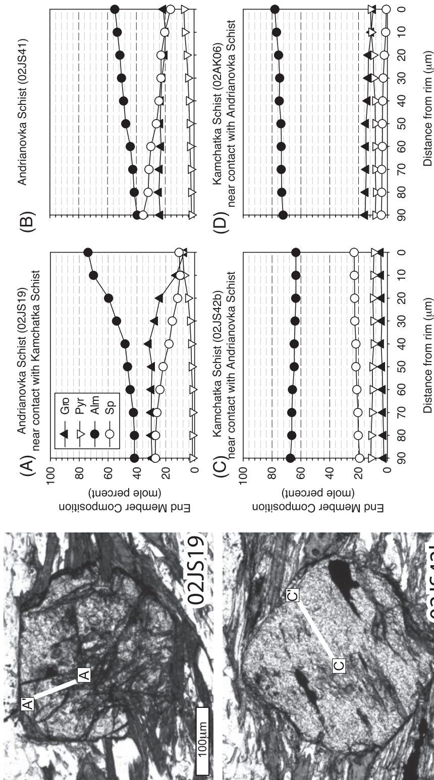
Fig. 6. Composition transects for garnets from the Andrianovka and Kamchatka schists. The photomicrographs show two of the analyzed grants and the transects for the analyses (white lines). End members were calculated from molar concentrations, with grossular (Gro) = \text{Ca}/(\text{Ca}+\text{Mn}+\text{Fe}+\text{Mg}) , almandine (Alm) = \text{Fe}/(\text{Ca}+\text{Mn}+\text{Fe}+\text{Mg}) , spessartine (Sp) = \text{Mn}/(\text{Ca}+\text{Mn}+\text{Fe}+\text{Mg}) , and pyrope (Py) = \text{Mg}/(\text{Ca}+\text{Mn}+\text{Fe}+\text{Mg}) .
