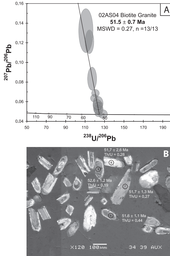
Fig. 17. Tera-Wasserburg concordia plot (panel A) and CL image (panel B) with ^{207}\text{Pb} -corrected ^{206}\text{Pb}/^{238}\text{U} grain-ages for analyzed representative zircons from a late syn-kinematic equigranular granite (Sample 02AS04) which stitches the Andrianovka Suture in the Krutogorova river region. Isotopic data are presented in Appendix A.11. The zircons yield a weighted mean ^{207}\text{Pb} -corrected ^{206}\text{Pb}/^{238}\text{U} age of 51.5 \pm 0.7 Ma coeval with peak condition and anatexis at deeper structural levels.
