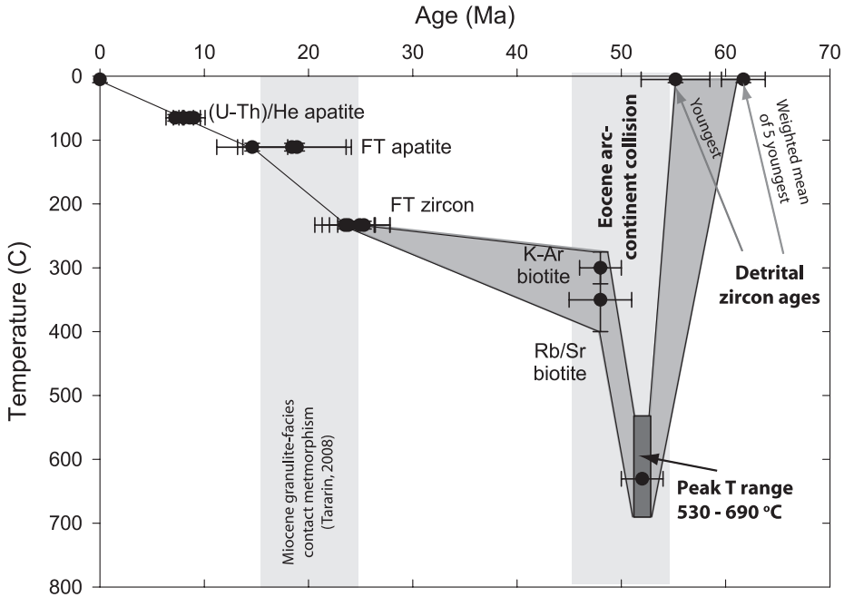
Fig. 24. Time-temperature history for Sredinnyi Complex. Data sources used for construction of this plot are given in table 3. Subduction and metamorphism of sediments as young as Paleocene in age resulted in high-grade metamorphism and migmatization at the deepest exposed structural levels. This high-grade event is well-constrained by monazite and zircon geochronology at ~52 Ma. Temperatures and pressures are from this study (after Khanchuk, 1985) and Tamarin (2008). Cooling of core rocks to below ~300°C appears rapid. Low-temperature thermochronometry indicates that subsequent cooling proceeded more slowly.
