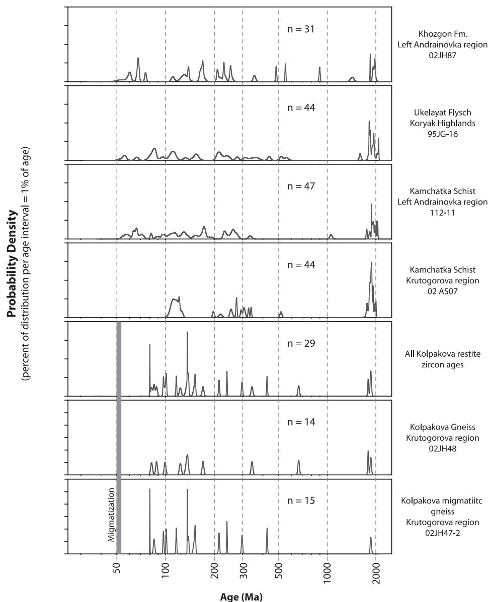
Fig. 22. Probability density plots for all detrital and metasedimentary zircon grain-ages. The age data are in log scale. A log-normal Gaussian kernel algorithm with an \alpha = 0.6 (Brandon, 1996) is used for the construction of grain-age probability density (PD) plots. PD plots are shown on log scale to accommodate the broad age range exhibited by these samples.
