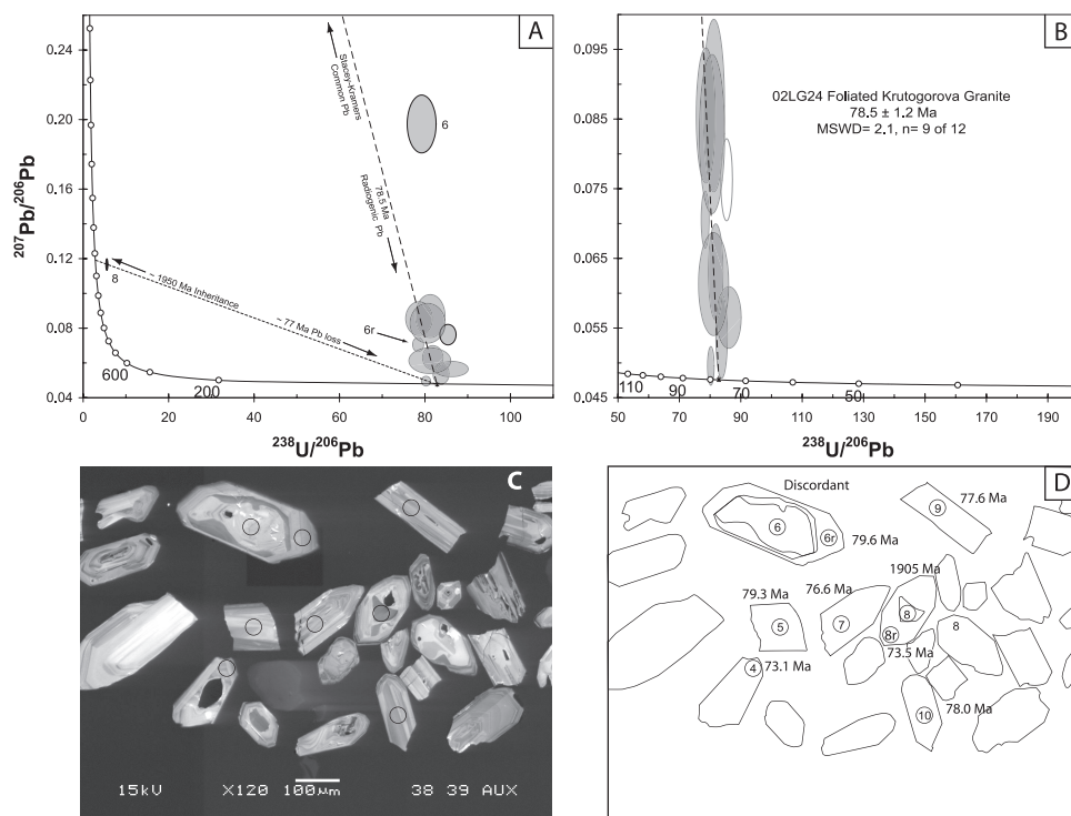
Fig. 9. Single-grain U-Pb data and CL images for zircons from the foliated Krutogorova Granite (sample 02LG24) in the upper Krutogorova watershed. Expanded (A) and focused (B) Tera-Wasserburg concordia diagrams show data defining a linear array of analyses from model common Pb (Stacey and Kramers, 1975) to radiogenic lead at 78.5 \pm 1.2 Ma. CL images (C) display relative textural homogeneity, although a few grains do contain apparent inherited cores. Analysis of an apparent core in grain #8 (D) yields a ^{204}\text{Pb} -corrected ^{207}\text{Pb}/^{206}\text{Pb} age of 1905 Ma, while the corresponding rim gives a ^{207}\text{Pb} corrected ^{206}\text{Pb}/^{238}\text{U} age of 73.5 \pm 2.3 Ma (Appendix A.3). The age data are consistent with partial assimilation of Kolpakova gneiss protolith, during pluton emplacement at 78 Ma. The 1.9 Ga grain-age component is well-represented among detrital zircons of the Kolpakova Gneiss and Kamchatka Schist.
