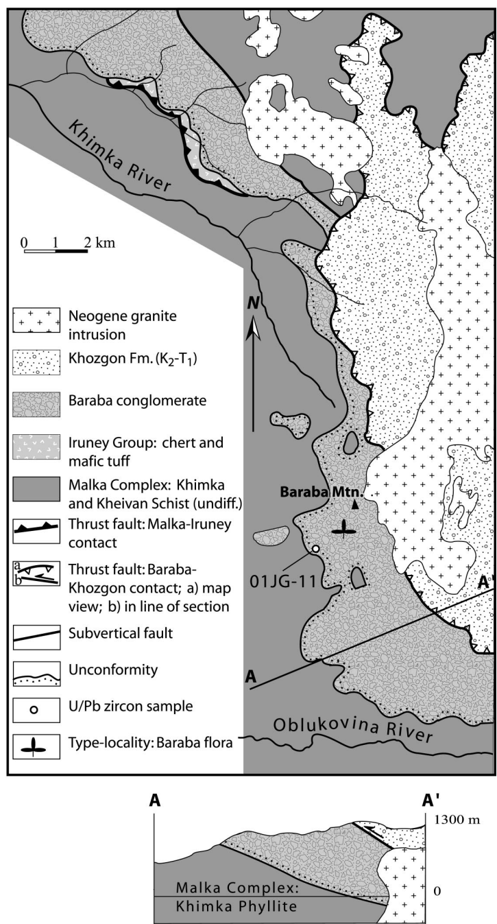
Fig. 18. Simplified geologic map and cross-section of the Baraba Mountain region (Soloviev and others, 2004). The unconformity between phyllites of the Malka Complex and the unroofing sequence of the Baraba conglomerate provides an important age constraint on metamorphism. Based on floral stratigraphy the Baraba conglomerate has traditionally been assigned a Campanian-Maastrichtian age (Shapiro and others, 1986). A 50.5 \pm 1.2 Ma U-Pb zircon age from a basal tuff horizon indicates deposition occurred after the Early Eocene.
