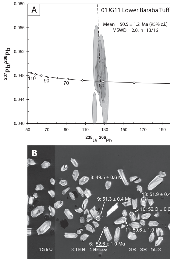
Fig. 19. Tera-Wasserburg concordia plot (panel A) and CL image (panel B) with ^{207}\text{Pb} -corrected ^{206}\text{Pb}/^{238}\text{U} grain-ages for analyzed representative zircons from the lower tuffaceous member of the Baraba Conglomerate (sample 01JG11) which unconformably overlies low greenschist facies rocks of the Malka Complex. Isotopic data are presented in Appendix A.12. The zircons yield a weighted mean ^{207}\text{Pb} -corrected ^{206}\text{Pb}/^{238}\text{U} age of 50.5 \pm 1.2 Ma indicating that exhumation of Malka Complex rocks was nearly synchronous with peak conditions at depth.
