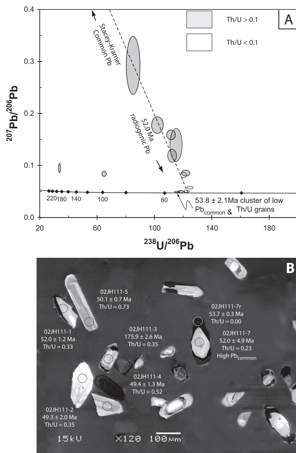
Fig. 16. Tera-Wasserburg concordia plot (panel A) and CL image (panel B) with ^{207}\text{Pb} -corrected ^{206}\text{Pb}/^{238}\text{U} grain-ages for analyzed representative zircons from granite intrusion (sample 02JH111) within the Kolpakova Gneiss in the Left Andrianovka region. The data exhibit considerable complexity and three populations can be identified: 1) a high common Pb, moderate Th/U population with a ~52 Ma weighted mean ^{207}\text{Pb} -corrected ^{206}\text{Pb}/^{238}\text{U} ages; 2) a low common Pb, low Th/U, high U rims with a 53.8 \pm 2.1 Ma age; and 3) two zircon with low common Pb, moderate Th/U that plot off the radiogenic-common Pb mixing line interpreted as discordant xenocrystic cores (Appendix A.10).
