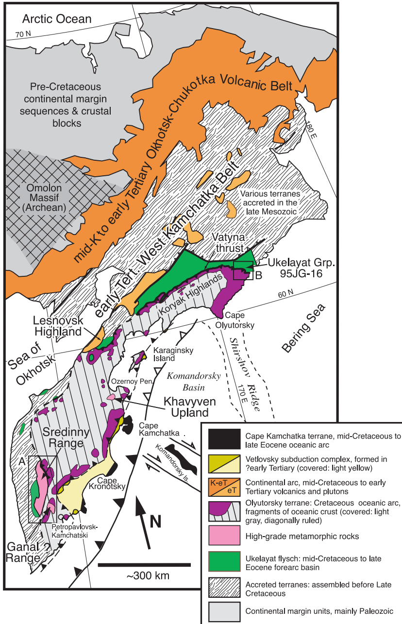
Fig. 1.(B) Generalized tectonic map of the Kamchatka Peninsula and Koryak Highlands. Medium to high-grade metamorphic rocks crop out in the Sredinnyi, Ganal, and Khavyven Ranges (Tilman and Bogdanov, 1992; Shapiro, 1995). The Sredinnyi Complex is exposed as domal uplift within a tectonic window into the lower plate beneath regionally extensive Olyutorsky or Achaivayam-Valagin arc thrust sheet. Boxes show: (A) Area of detailed map of the Sredinnyi Range (fig. 2) and (B) 1995 field area and sampling region for Ukelayat Group detrital zircon sample (95JG-16).
