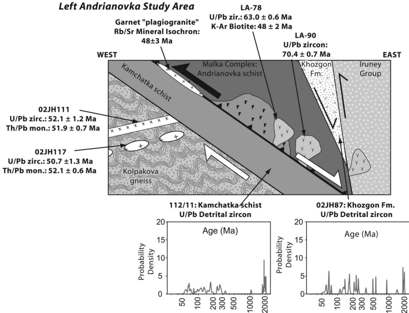
Fig. 25. Simplified schematic sections of the Krutogorova and Left Andrianovka study areas summarizing the geochronologic data in the context of important structural and tectono-stratigraphic relationships.
