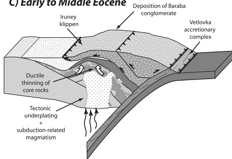
Fig. 26. Schematic model for the tectonic evolution of the Kamchatka Peninsula and the Sredinnyi Range in three time intervals.
