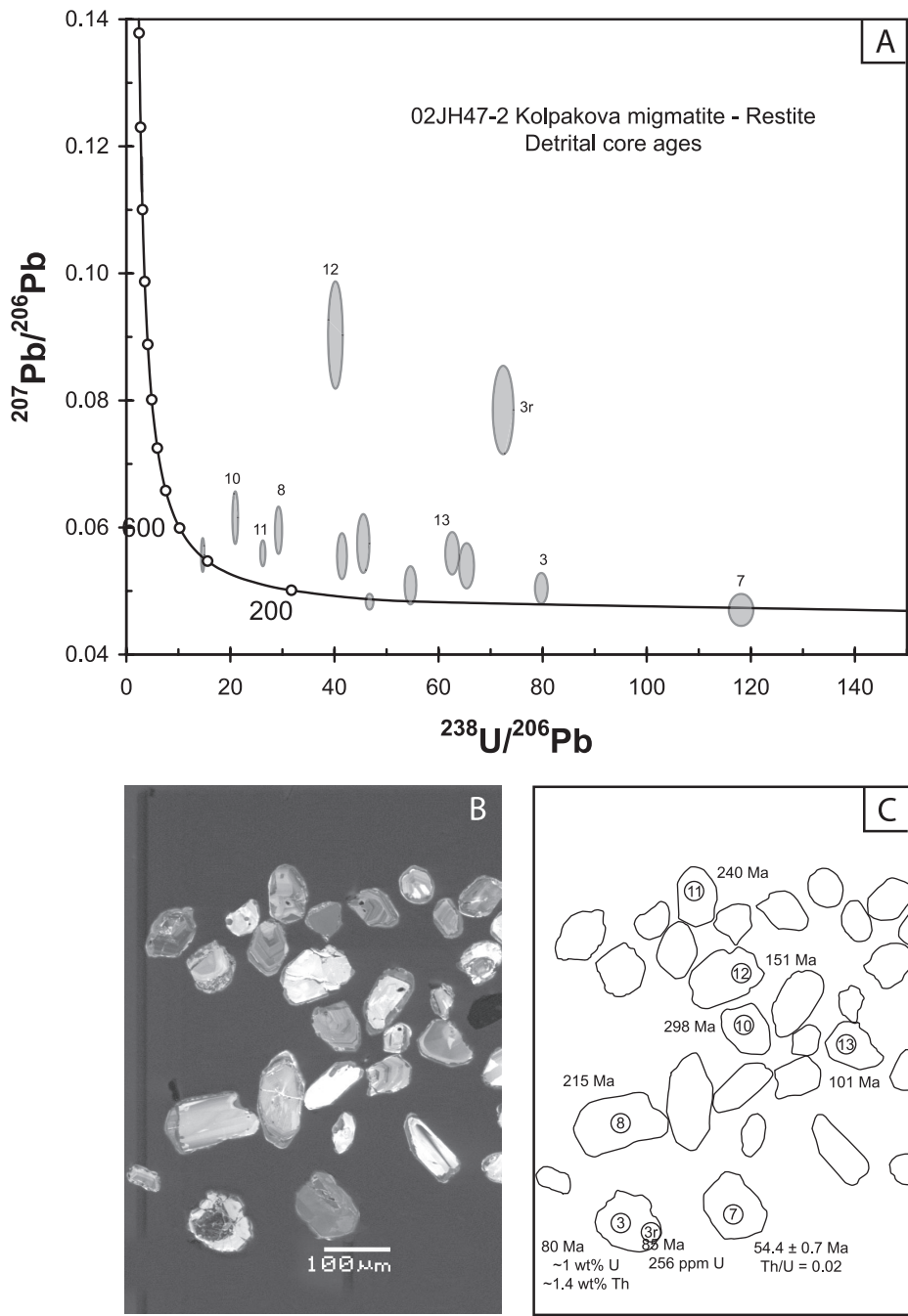
Fig. 7. (A) Tera-Wasserburg concordia plot of single-grain SHRIMP U-Pb analyses for sample 02JH47-2—a melanosome within migmatites of the Kolpakova Gneiss in the upper Krutogorova watershed (fig. 4). (B) Cathodoluminescence image of polished zircons in epoxy depicting the texturally heterogeneous nature of the zircon population. (C) Outlines of individual grains and the positions of spot analyses with corresponding ^{207}\text{Pb} -corrected ^{206}\text{Pb}^*/^{238}\text{U} ages. Encircled numbers refer to isotopic data in Appendix A.1.
